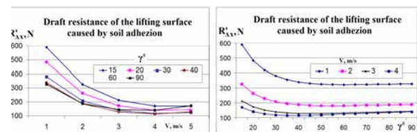
Fig. 4. Draft resistance of the lifting surface caused by soil adhesion depending on speed v and the inclination angle \gamma of the horizontal generatrix.
