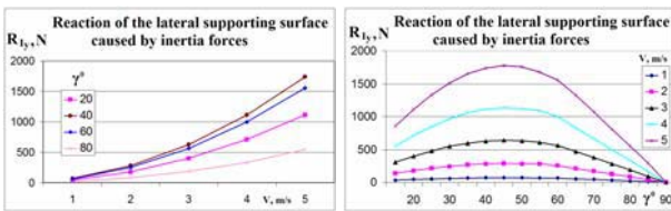
Fig. 8. Reaction of the lateral supporting surfaces caused by soil inertia forces depending on speed v and the inclination angle \gamma of the horizontal generatrix.
