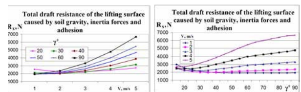
by soil gravity, inertia forces and adhesion depending on speed v and the inclination angle \gamma of the horizontal generatrix.
