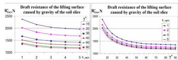
Fig. 2. Draft resistance of the lifting surface caused by the gravity of the soil slice depending on speed v and the inclination angle \gamma of the horizontal generatrix.
