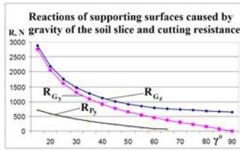
Fig. 6. Reactions of the lower and lateral supporting surfaces caused by gravity of the soil slice and share cutting resistance depending on the inclination angle \gamma of the horizontal generatrix.
