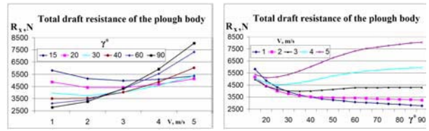
Fig. 11. Total draft resistance of the plough body depending on speed v and the inclination angle \gamma of the horizontal generatrix.
