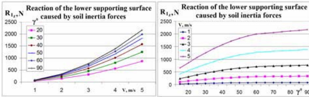
Fig. 7. Reaction of the lower supporting surface caused by soil inertia forces depending on speed v and the inclination angle \gamma of the horizontal generatrix.
