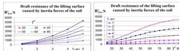
Fig. 3. Draft resistance of the lifting surface caused by the soil inertia forces of the soil slice depending on speed v and the inclination angle \gamma of the horizontal generatrix.
