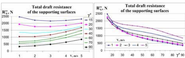
depending on speed v and the inclination angle \gamma of the horizontal generatrix.
