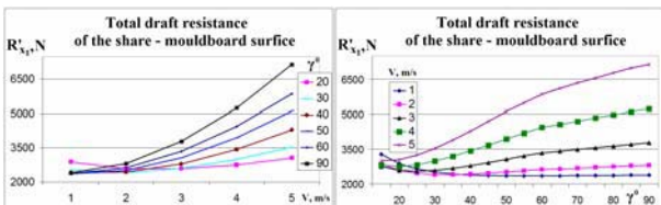
Fig. 9. Total draft resistance of the share-mouldboard surface caused by soil gravity, inertia forces, adhesion and share cutting resistance depending on speed v and the inclination angle \gamma of the horizontal generatrix.
